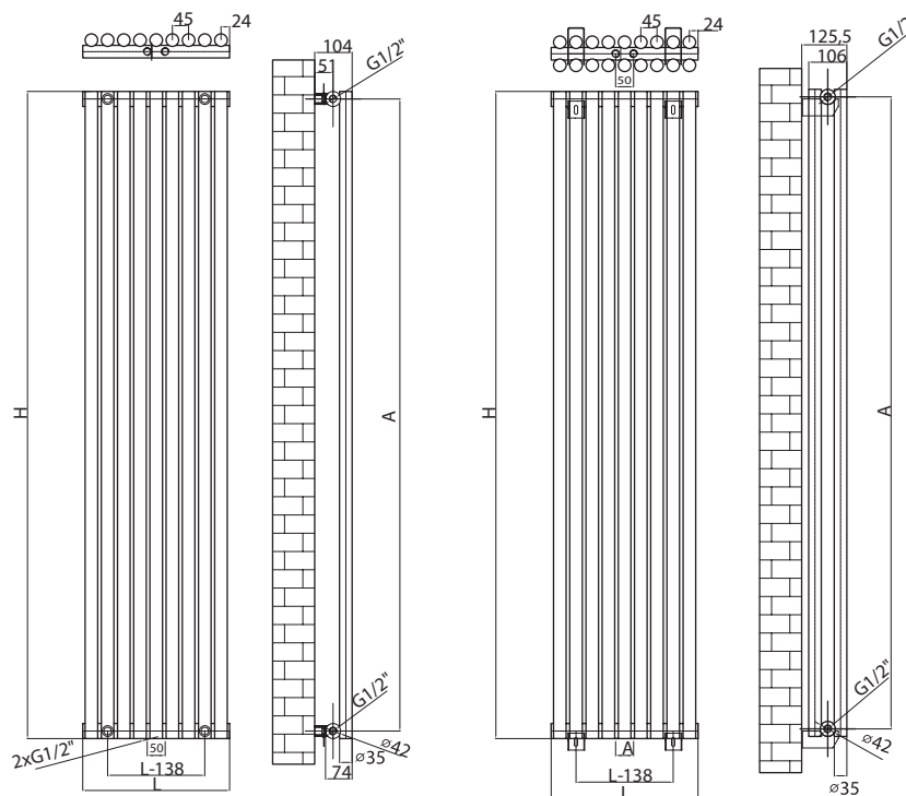
Hydraulic connections/ Conexiuni hidraulice
